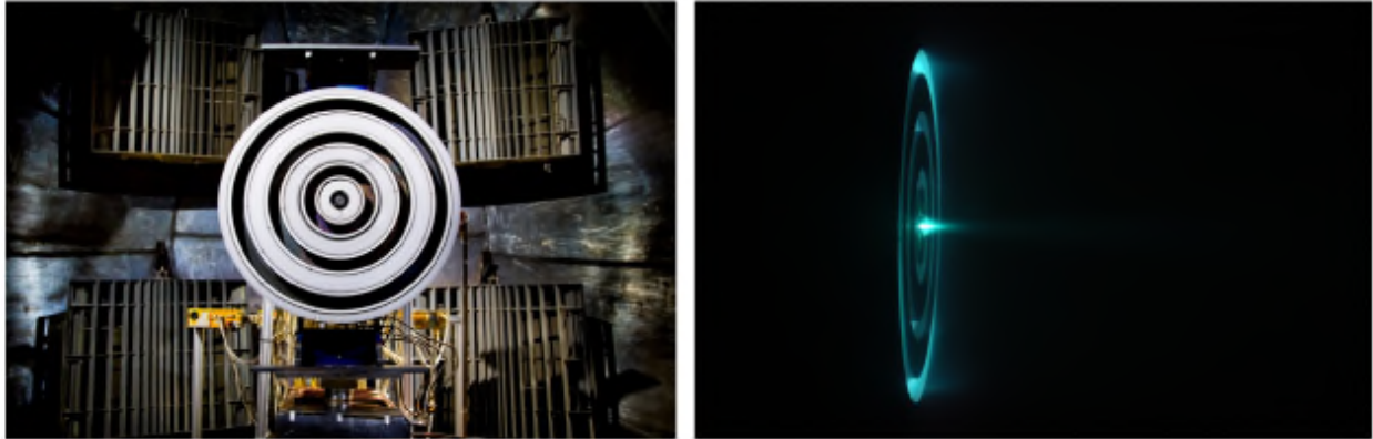
Figure 6. Photographs of X3 installed in University of Michigan's LVTF (left) and operating three channels simultaneously at 30 kW (right).
