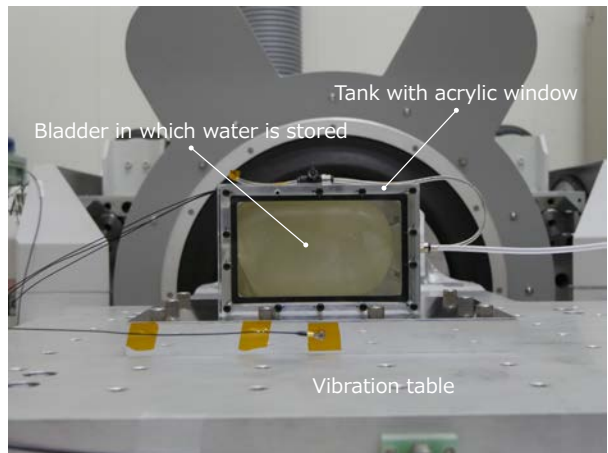
Figure 8. Configuration of the tank and the bladder vibration test
