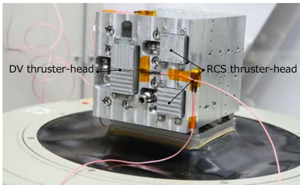
Figure 10. Configuration of the thruster-head vibration test
