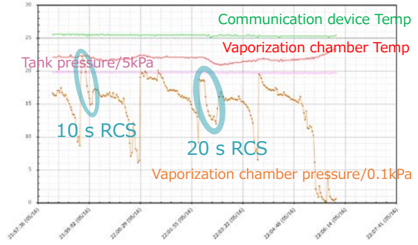
Figure 7. Coupling operation of the DV thrust and RCS thruster
