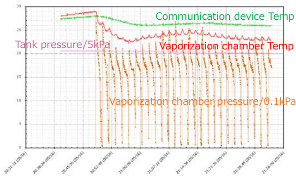
Figure 6. One-hour operation test result of the DV thruster
