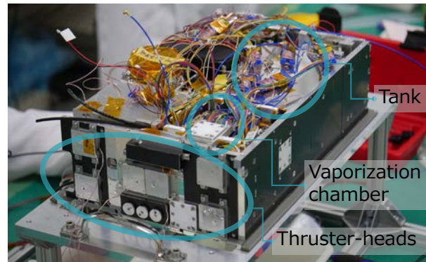
Figure 3. AQUARIUS integrated on EQUULEUS
