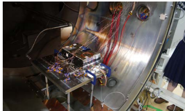
Figure 5. Operation test in the vacuum chamber by using whole systems of EQUULEUS
